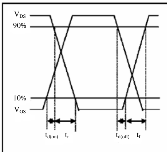
Switching Time Waveform
